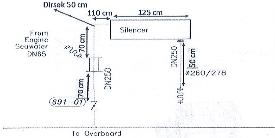
MAIN ENGINE
